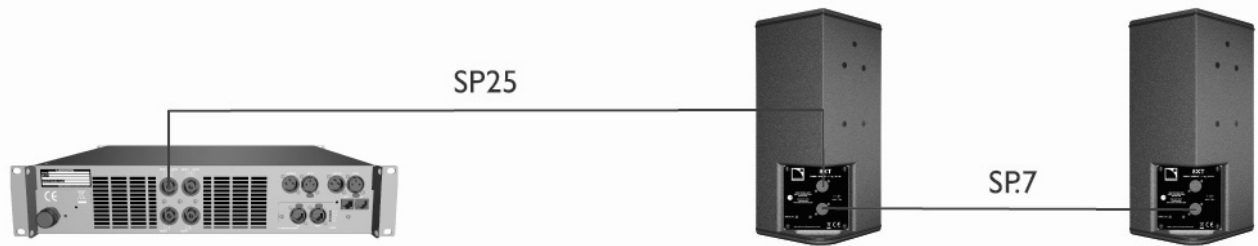
Figure 3: Connecting two 8XT in parallel to an LA4 amplified controller
