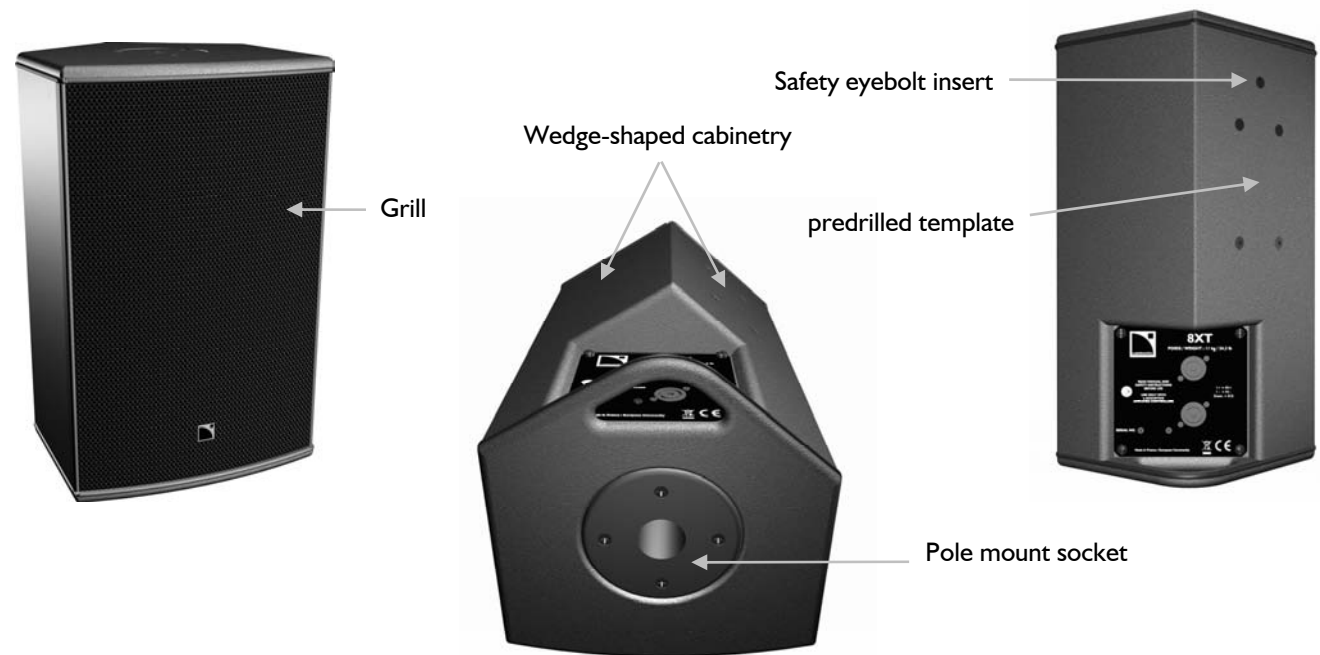
Figure 2: 8XT enclosure with rigging components
