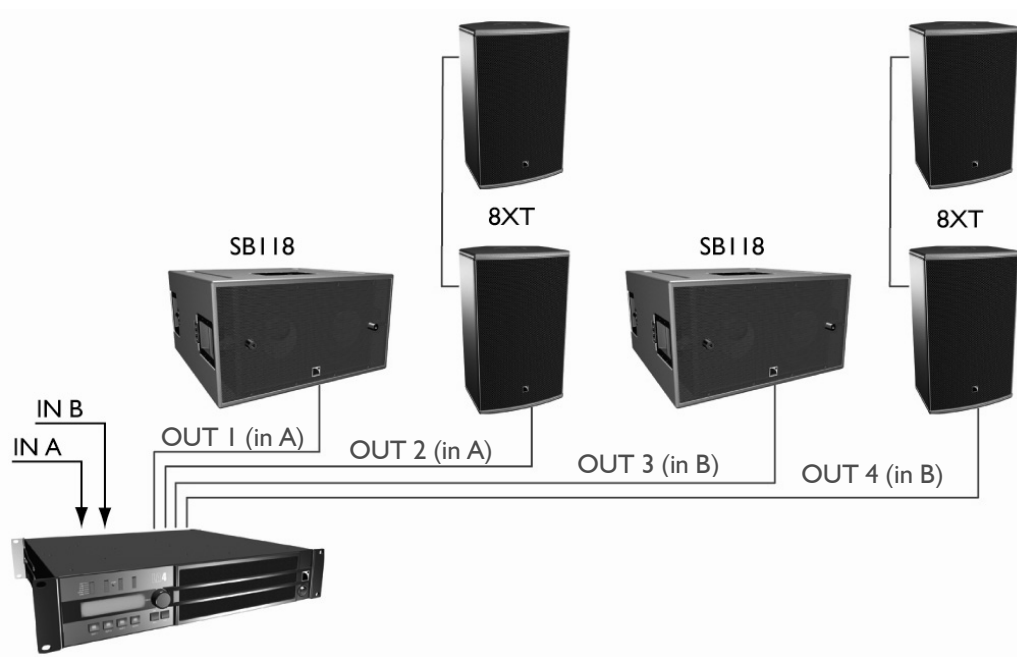
Figure 6: Two SBI 18 subwoofers and four 8XT enclosures connected to an LA4 controller
