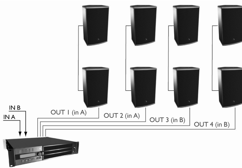
Figure 4: Eight 8XT enclosures connected to an LA4 controller
